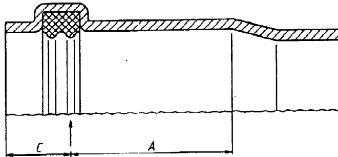
Figure 5: Effective sealing point
