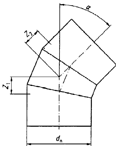
Figure 10: Bend, butt fused from segments
