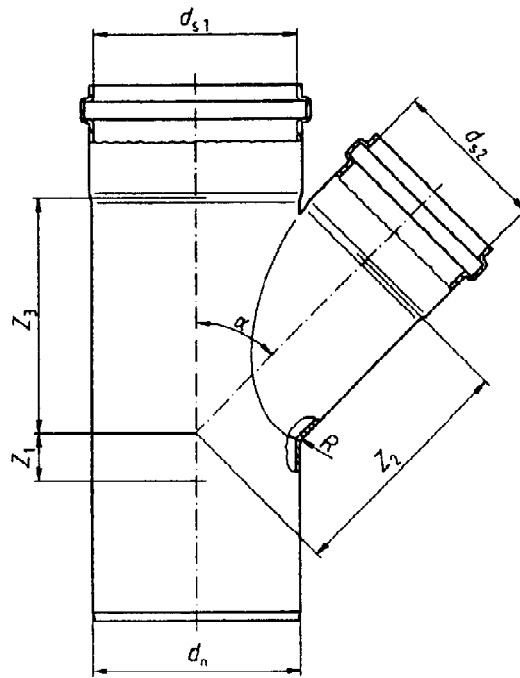
Figure 13: Reducing branch (unswept)
