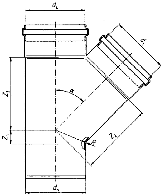
Figure 12: Branch (unswept)
