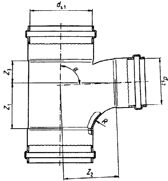
Figure 15: Reducing branch with all sockets (swept)
