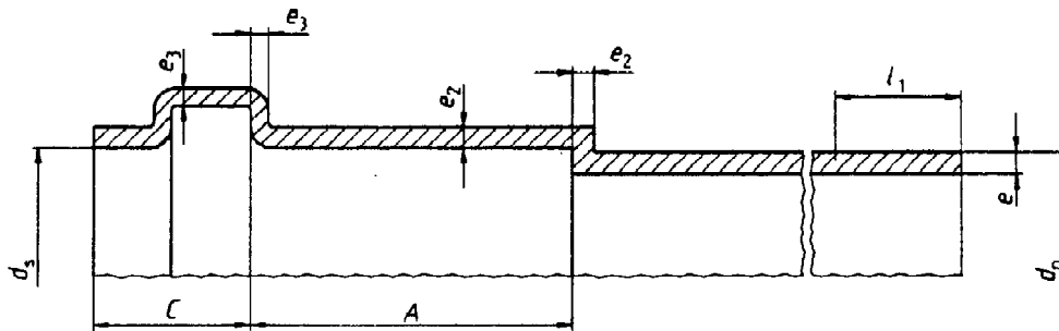
Ring seal socket with chamfer
