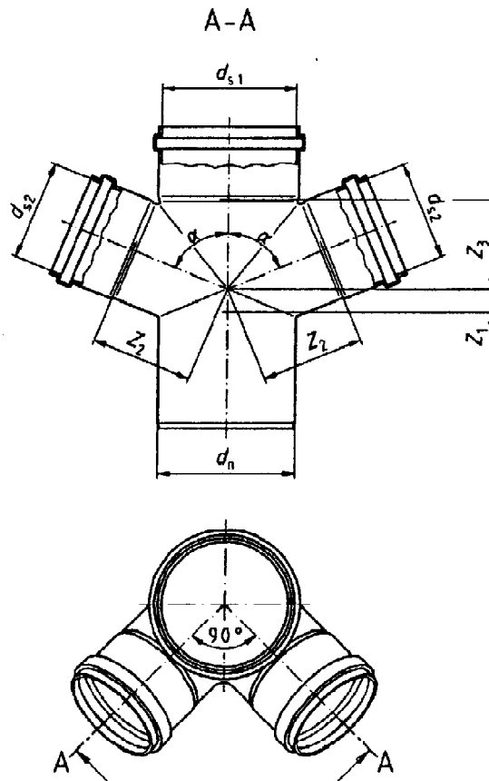
Figure 15: Reducing branch with all sockets (swept)
