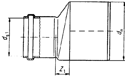
Figure 18: Reducer
