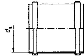
Figure 21: Repair collar
